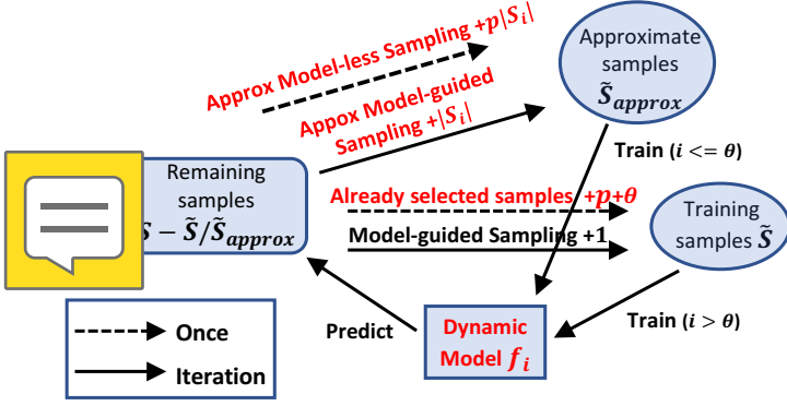
Fig. 3: FIST framework.
